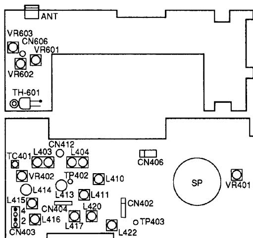
TX-RX UNIT (B/5)
