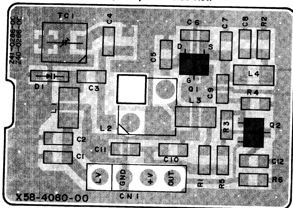
VCO UNIT (X58-4080-00) Component side view
